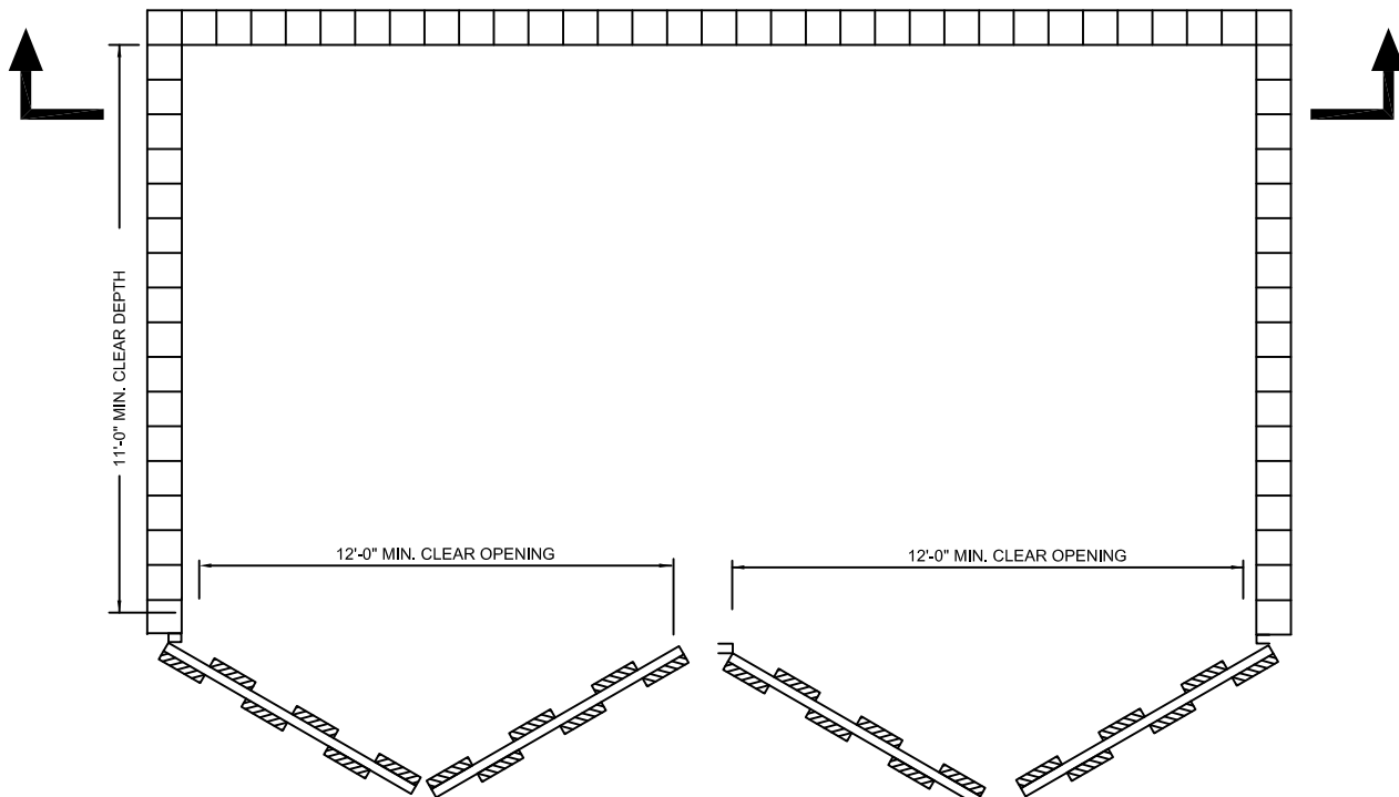
PLAN VIEW
