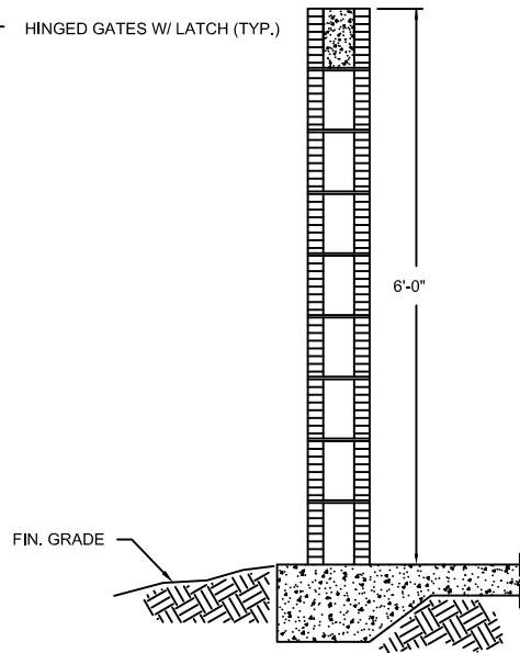
WALL SECTION
