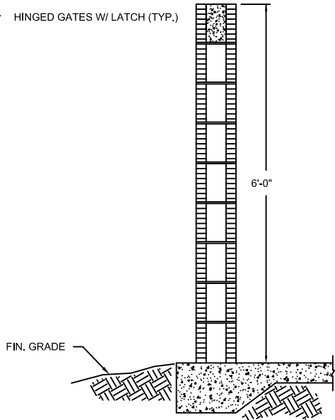
WALL SECTION
